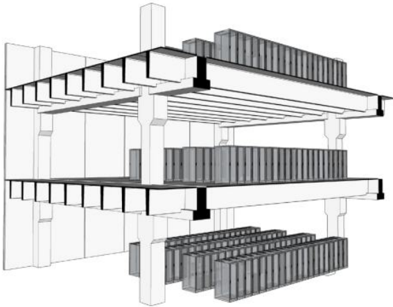
MODEL OF PREFABRICATED DATA CENTER WITH LONG CLEAR SPANS, FOR COLUMN FREE WHITE SPACE.
